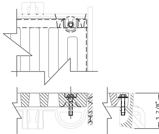
FRAME & GRATE SHOWING DEBRIS CHUTE SCALE 1:4
