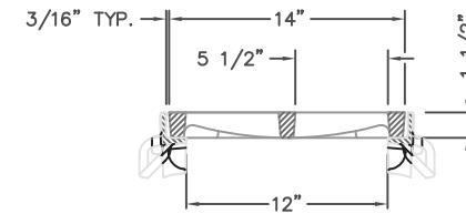
R-4999-DX TYPE "A" GRATE w/ TYPE "B" FRAME TYPICAL SECTION
